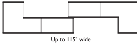
expando storage unit: cherry, 59"w x 17.75"d x 41.25"h
